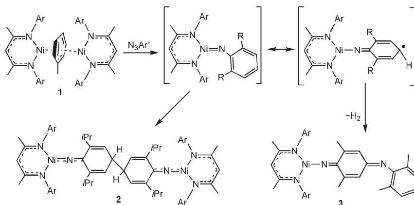
Scheme 1. Formation of 2 and 3 from 1 . Ar = 2,6- i Pr 2 C 6 H 3 ; Ar' = 2,6- i Pr 2 C 6 H 3 or 2,6-Me 2 C 6 H 3 .
