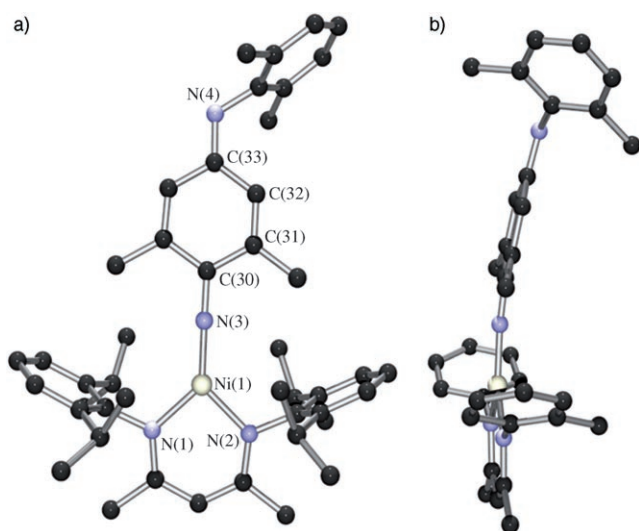
Figure 2. Pov-ray drawing of 3 ; (a) and (b) are orthogonal views. Hydrogen atoms are omitted for clarity. C black, N light blue, Ni white. Selected bond lengths [Å] and angles [°]: Ni(1)–N(3) 1.699(3), Ni(1)–N(1) 1.860(3), Ni(1)–N(2) 1.863(3), N(3)–C(30) 1.289(4), N(4)–C(33) 1.299(5); N(3)–Ni(1)–N(1) 133.46(13), N(3)–Ni(1)–N(2) 132.05(12), N(1)–Ni(1)–N(2) 94.44(12), C(30)–N(3)–Ni(1) 175.0(3), C(33)–N(4)–C(38) 120.9(3).
