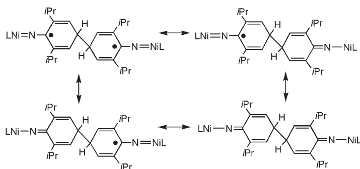
Scheme 2. Resonance forms of 3 . L = nacnac.
